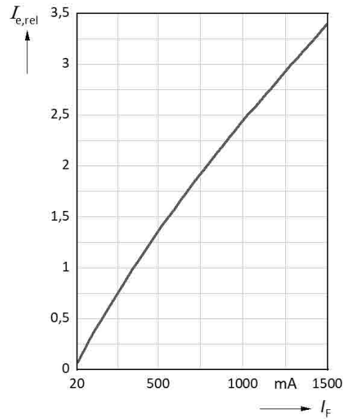
Relative Radiant Intensity vs. Forward Current
