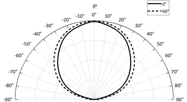
Radiation Pattern
