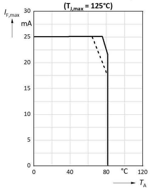
Forward Current vs. Ambient Temperature
