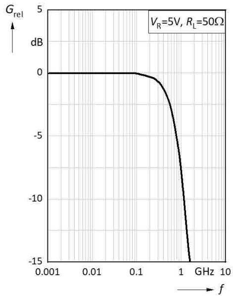
Frequency Response (Relative Gain vs. Frequency)
